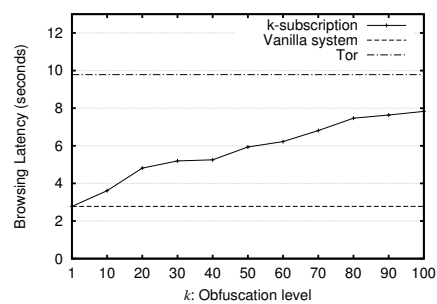
Figure 13: Browsing latency as a function of k when a user opens Twitter’s main page.
