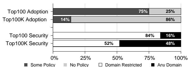
Figure 1: Global Alexa Top100, Top100K
