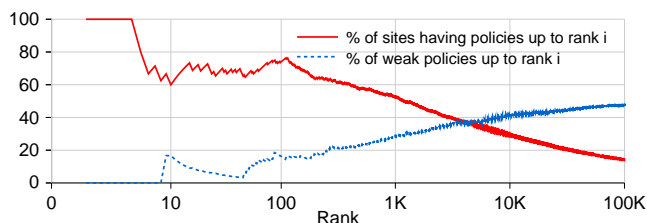
Figure 2: Correlation of policy adoption and security with site popularity rank.
