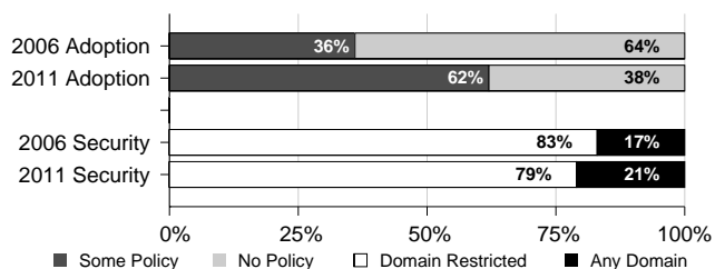
Figure 3: Alexa Top100 US
