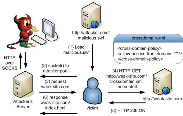
Figure 6: Attack Proxy Design
